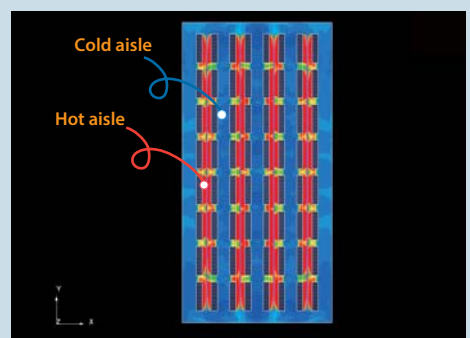
Fig. 4 Temperature Contour
