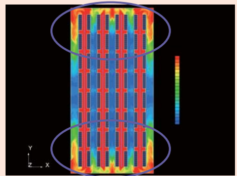
Fig.2 Temperature Contour Separated hot aisle and cold aisle
