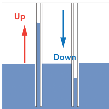
Figure 2: Capillary hydrophilic wall with plates of contact angle 60° (left) and water-shedding wall with plates of contact angle 120° (right)
