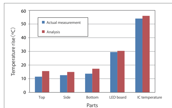
Temperature rise of each part
